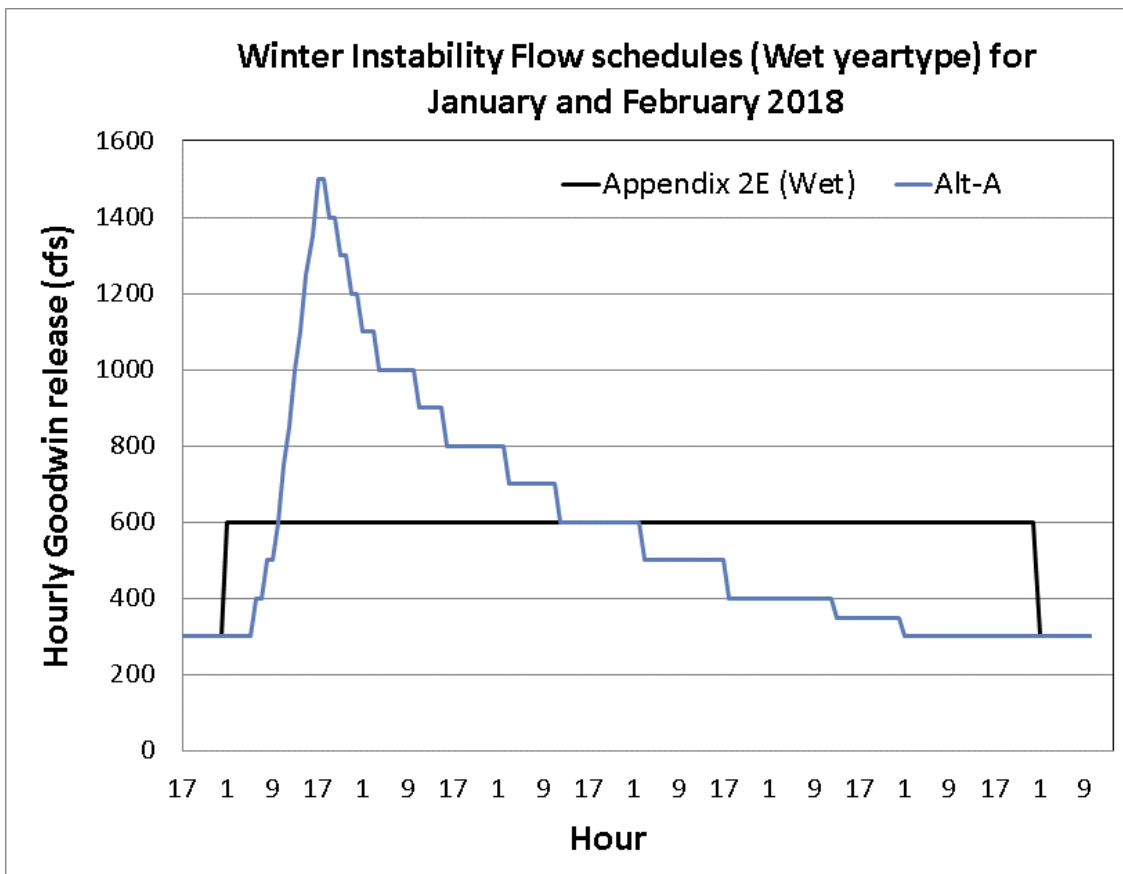
Figure 2-2. Stanislaus winter instability flow schedules (Wet yeartype) considered by SOG for January and February 2018. SOG advised, and NMFS approved, implementation of the “Alternative A” pulse flow schedule, though reservoir management releases from New Melones Reservoir.
