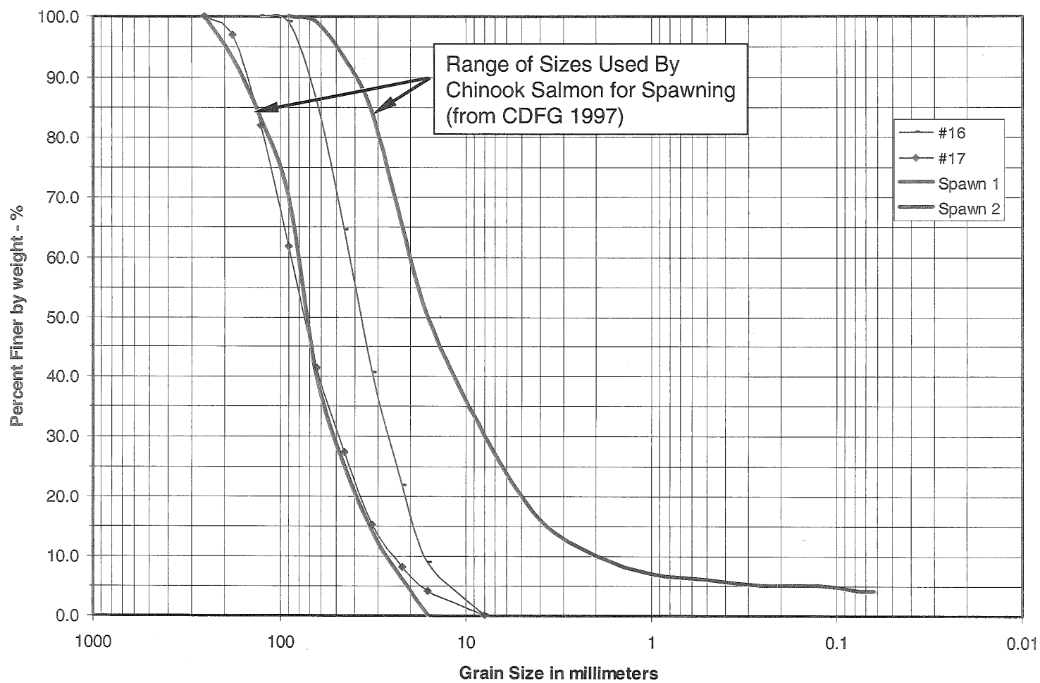
Grain Size Distribution Curve Samples 16 & 17 (DFG)
