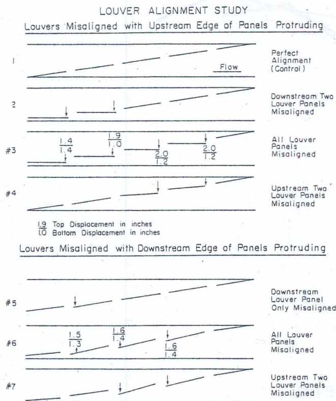
FIG. 25. Louver alignment configuration.
