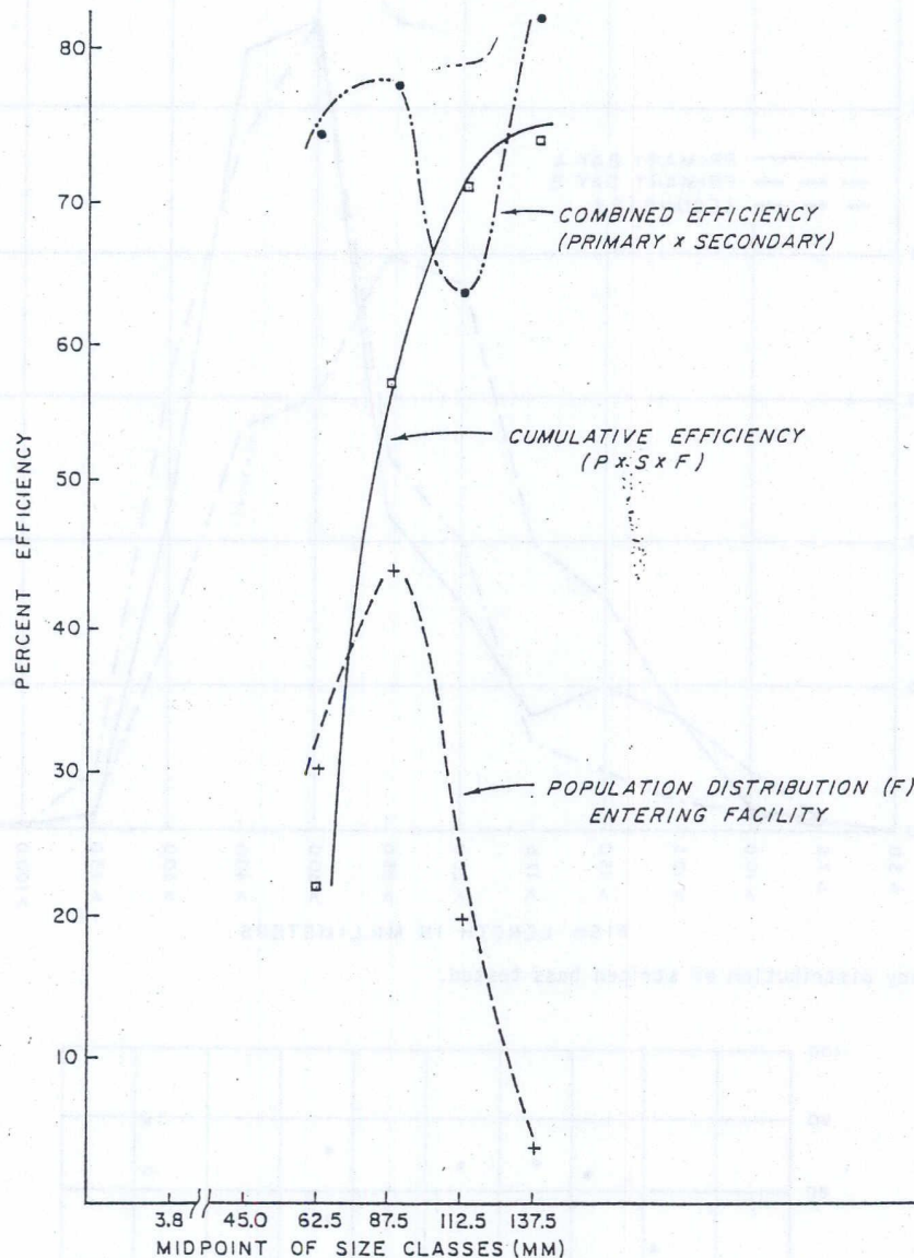
FIG. 15. Louver efficiency of the Delta Fish Protective Facility for king salmon (data for 1970-71 combined).
