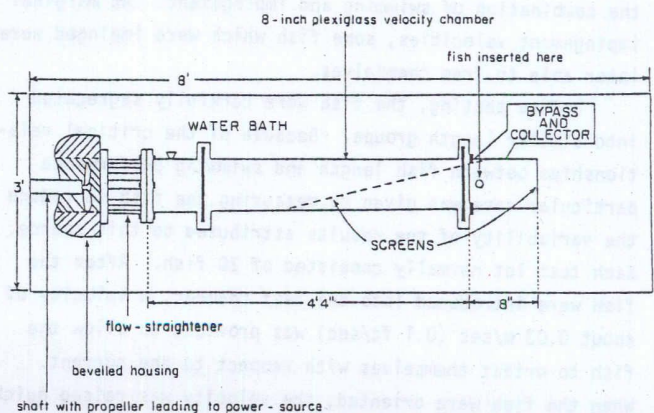
FIG. 2. Schematic diagram of velocity chamber.
